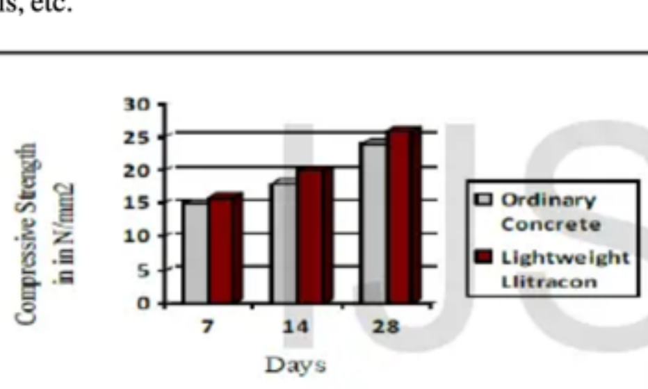
Fig 3: Compressive strength of the concrete [taken by (11)]
